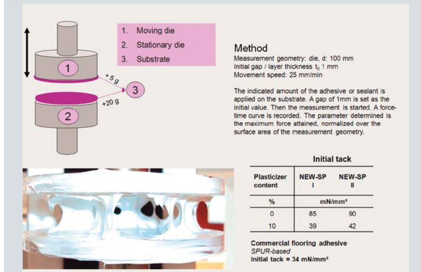
Figure 5: Method for evaluation of initial tack
